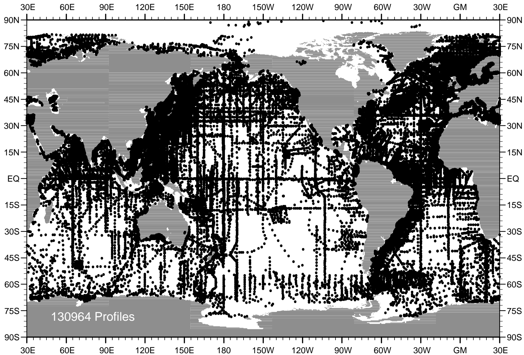
Distribution of pH Data
