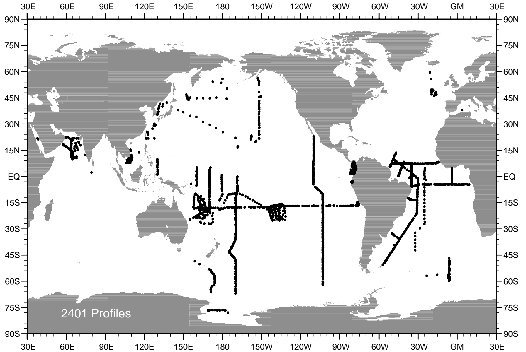
Distribution of TCO 2 and pH Data
